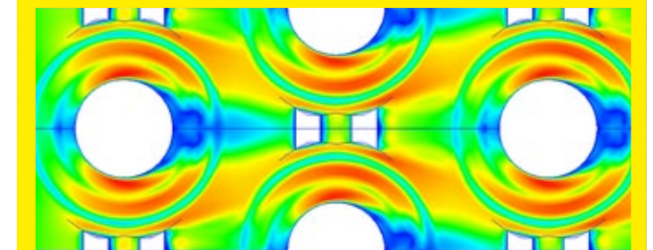
FLOW FIELDS BETWEEN FINS (CFD)
